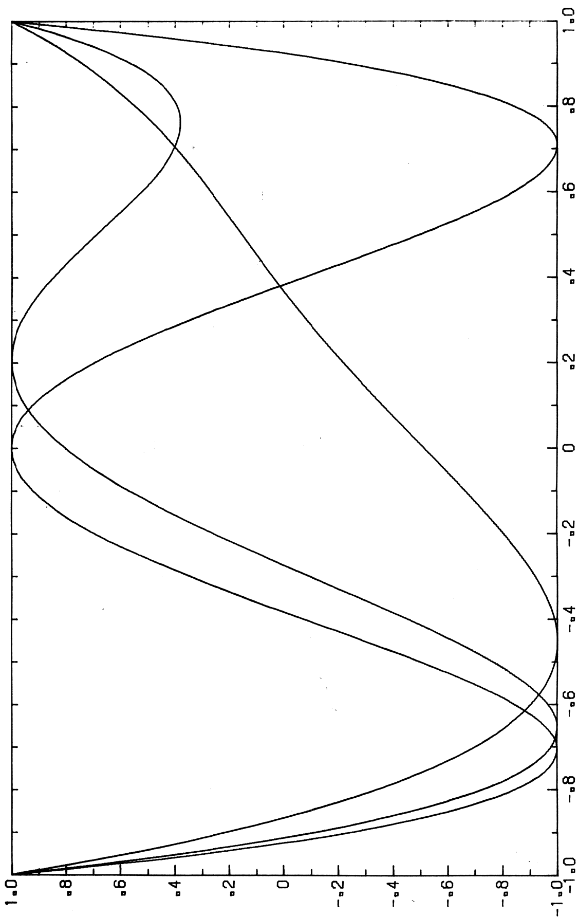
fig. 1.2. P_4\left(\frac{1}{2}^\beta(4,p)(x-1)\right) , p = 1, 2, 3 .
